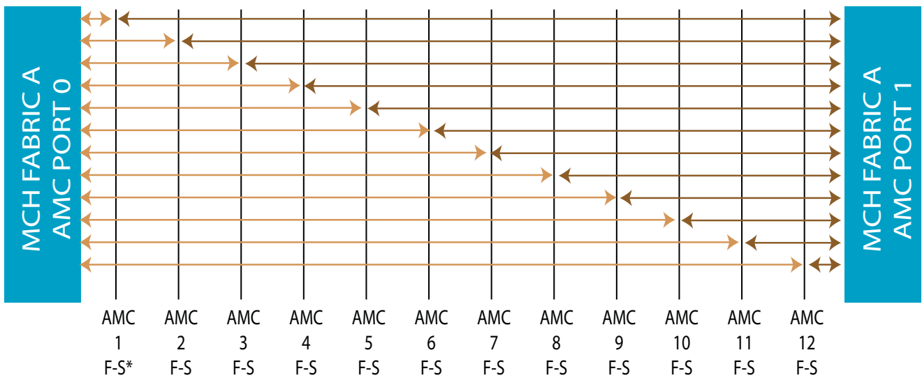
FIGURE 2. VT892 Topology for AMC Ports 0 and 1
