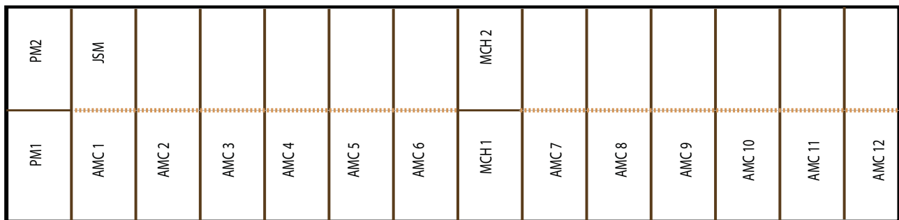
FIGURE 8. VT892 Slot locations
